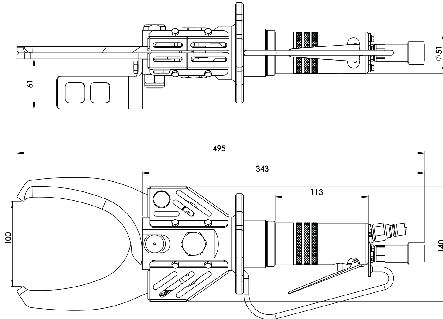
Dimensional drawing
