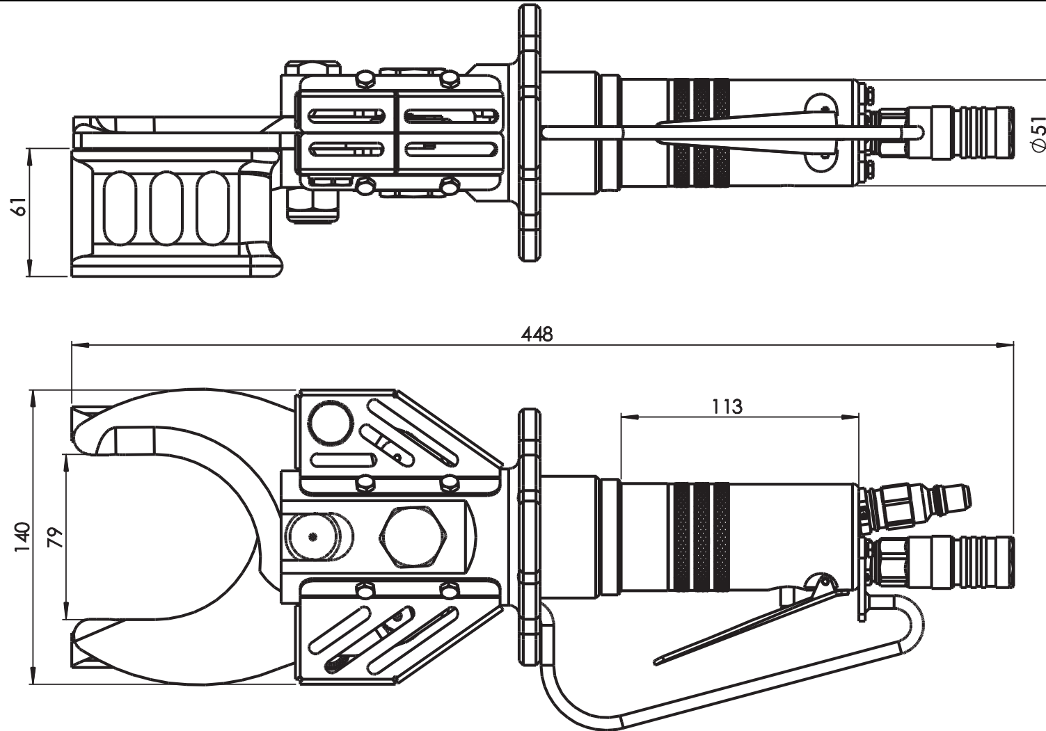
Dimensional drawing
